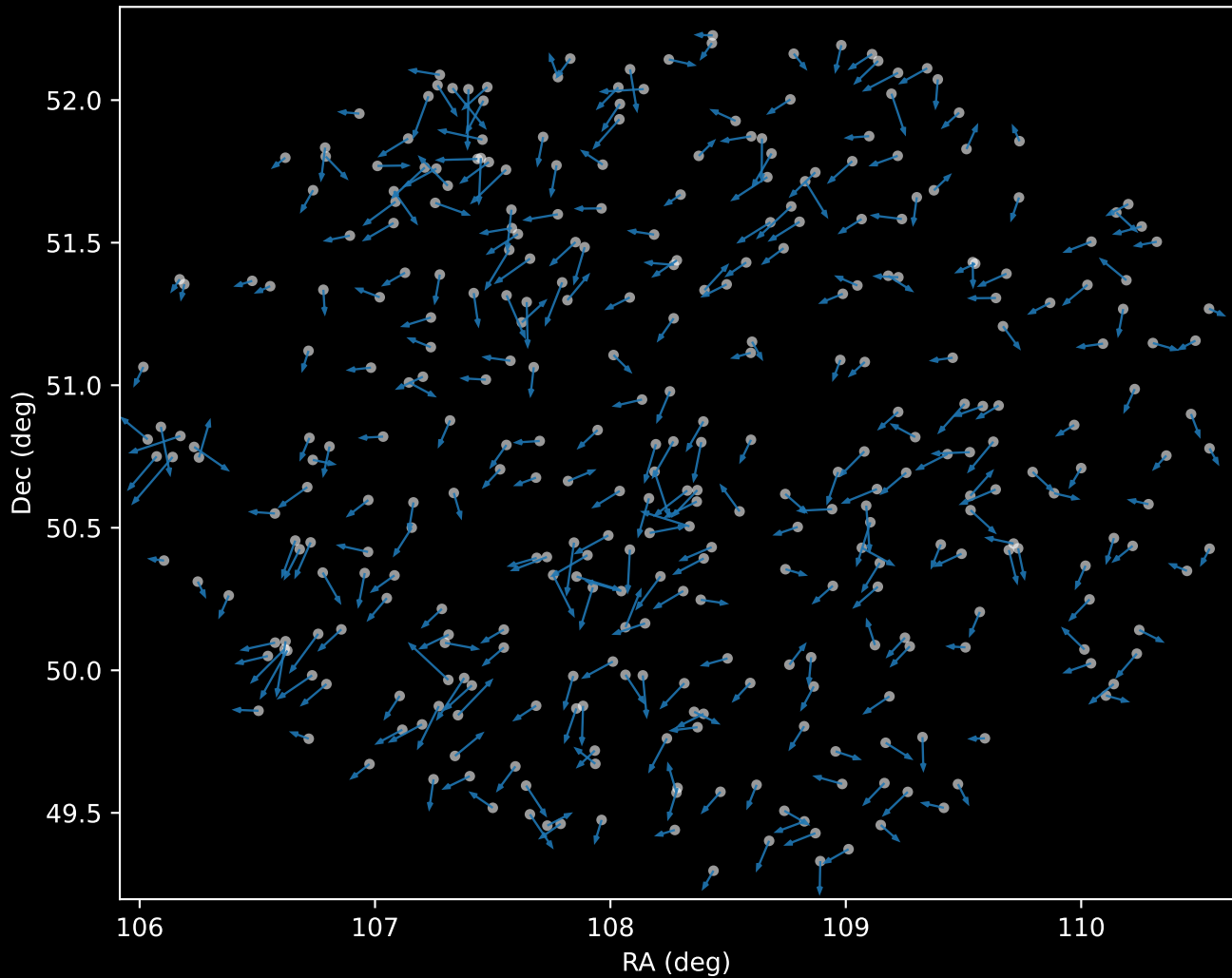
APOGEE DR17 Cluster 0 Proper Motion Vectors (n=344)
