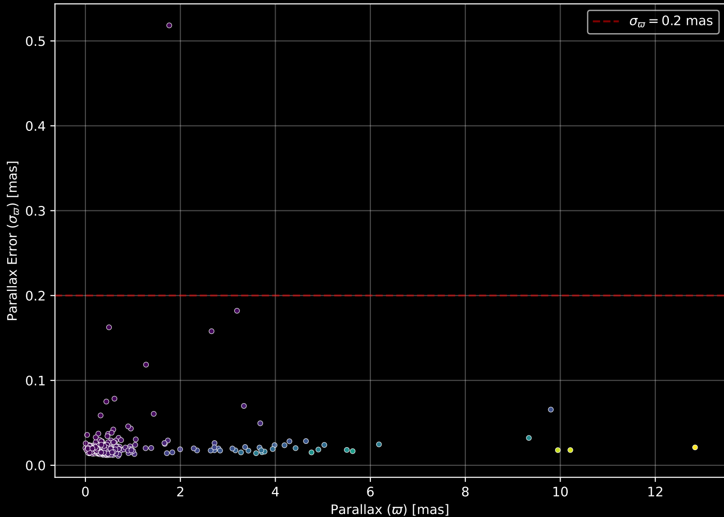
APOGEE DR17 Field: [120-12] Parallax Quality (n= 370)
