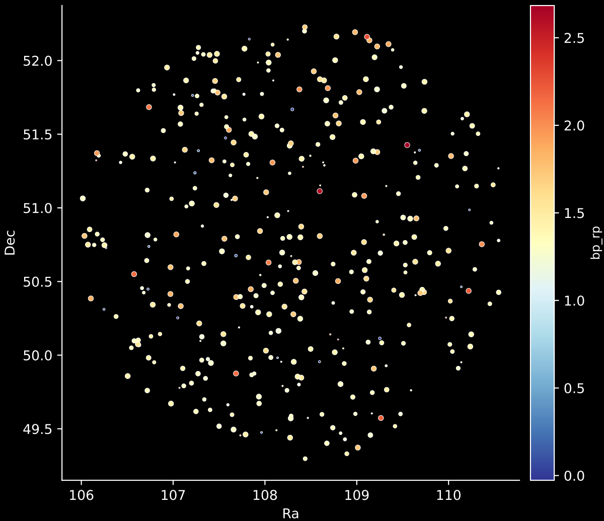
APOGEE DR17 Field: [120-12] Stars: 370
