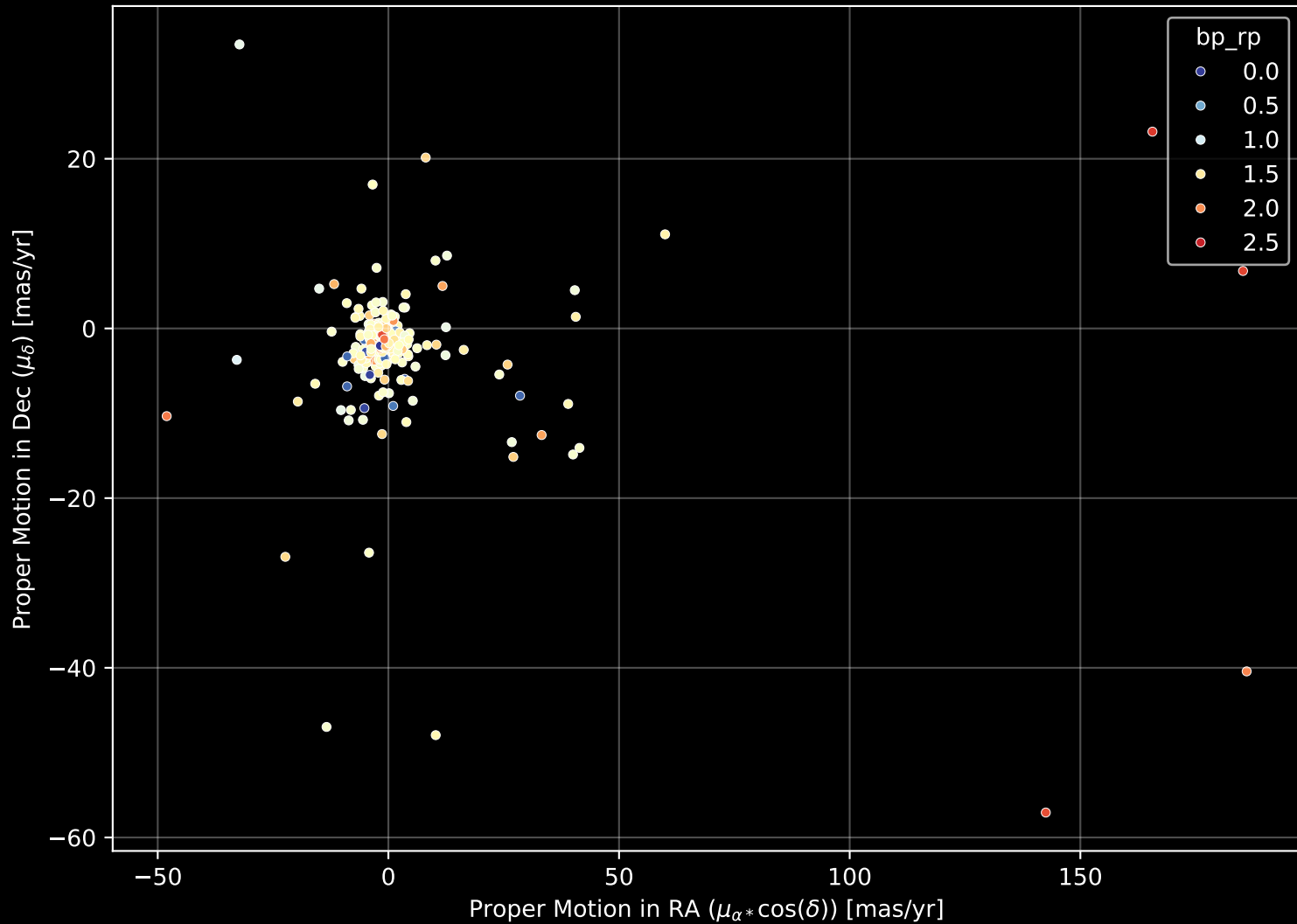
APOGEE DR17 Field: [120-12] Proper Motion Diagram (n= 370)
