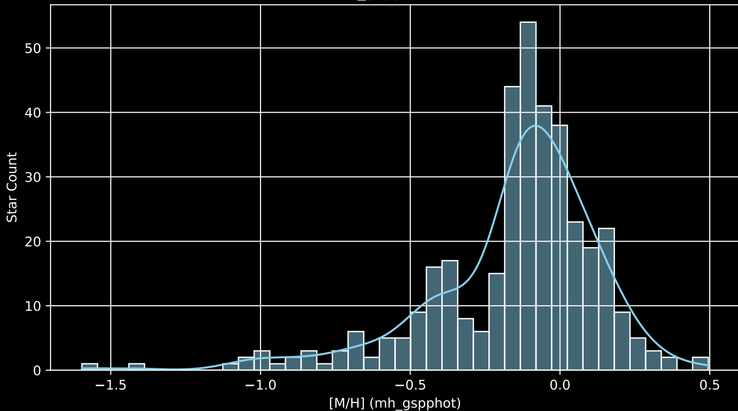
APOGEE DR17 Field: [120-12 [M/H] (mh_gspphot) (n= 369)
