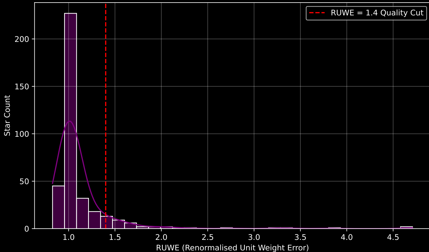
GAPOGEE DR17 Field [120-12] RUWE Distribution (n= 364)
